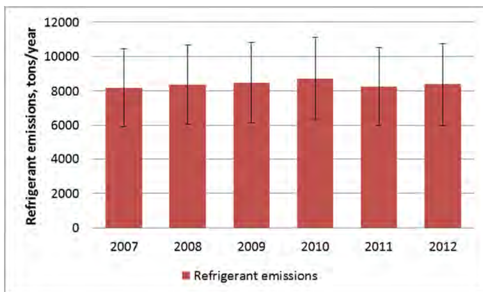
Figure 71 Estimated refrigerant emissions of the global fleet 2007–2012.
