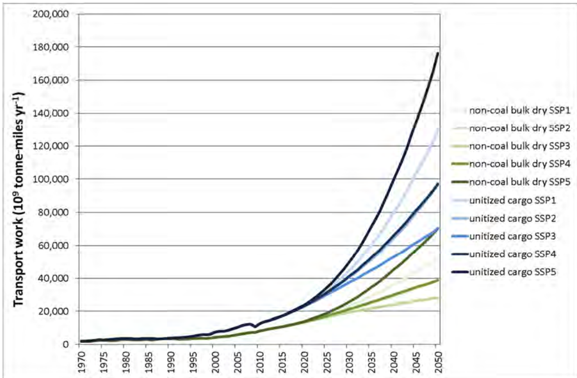
Figure 11: Historical data to 2012 on global transport work for non-coal combined bulk dry cargoes and other dry cargoes (billion tonne-miles) coupled to projections driven by GDPs from SSP1 through to SSP5 by 2050.
