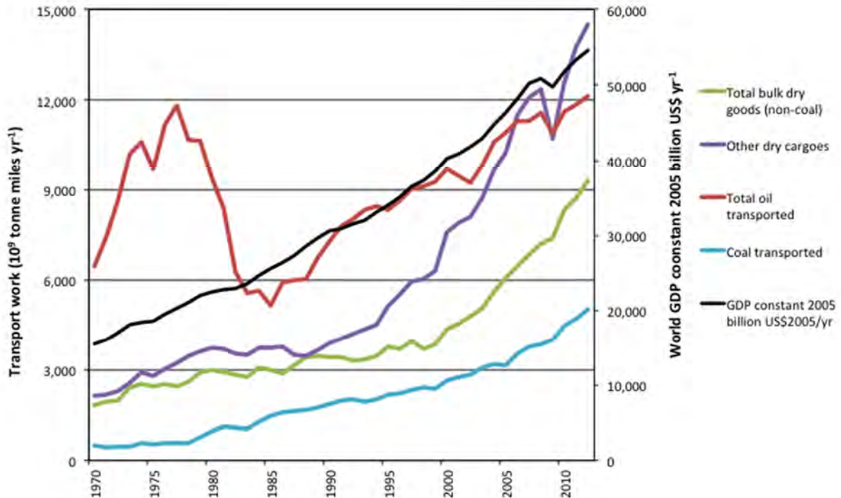
Figure 33: Transport work for all categories of cargo provided by UNCTAD, 1970 to 2012 in billion tonne-miles, also illustrated with global GDP (right hand axis) in billion US$ (constant 2005 prices).
