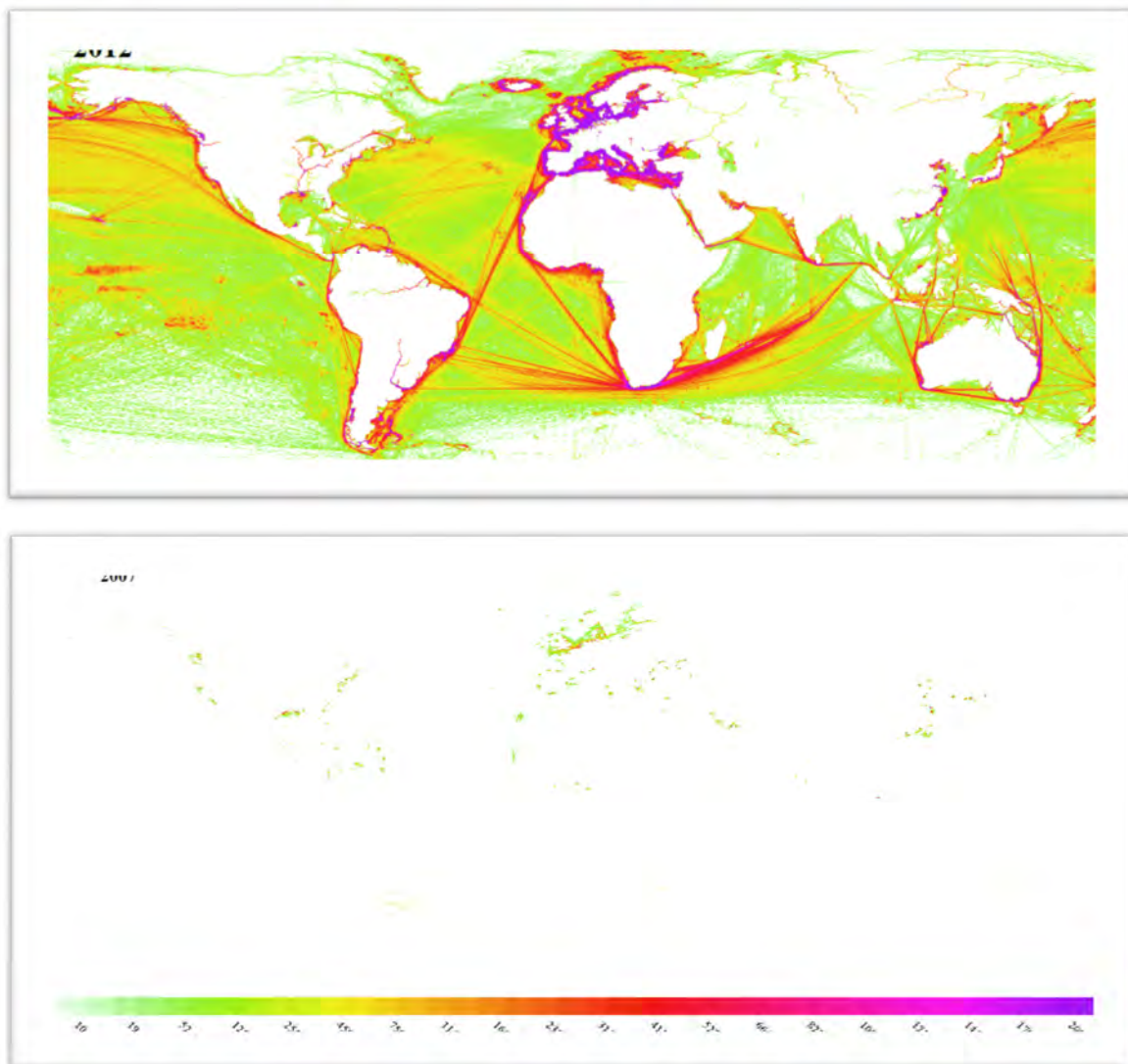
Figure 4: Geographical distribution of AIS-messages processed by the Pre-processor for 2007 and 2012. All available AIS-datasets have been combined. Unit: total amount of messages per grid cell with an area of 0.2 x 0.2 degrees. Both plots contains the same scale.
