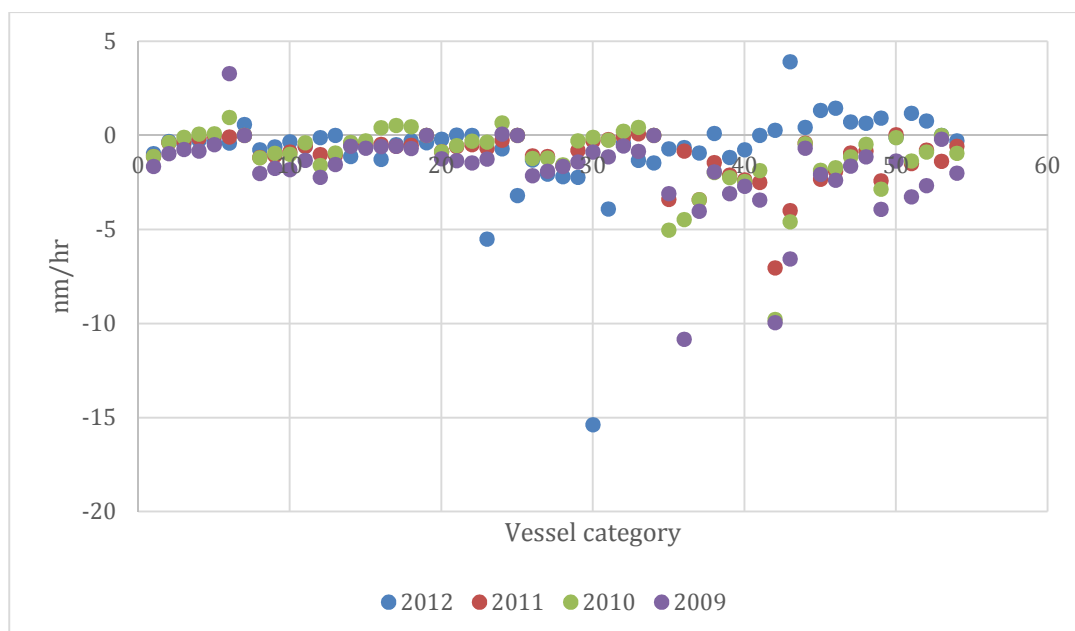
Figure 19: Difference between average speed at sea for each ship size and type category. Negative values indicate that LRIT provides a lower estimate of speed than the extrapolated AIS.
