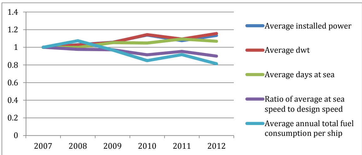
Figure 34 Average trends in the container sector 2007–2012, indexed to 2007.
