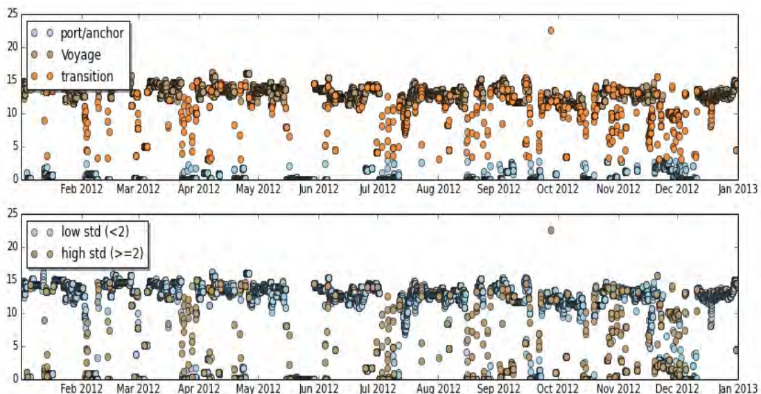
Figure 7: Characterisation of ship phases used in the extrapolation algorithm for an example vlcc ship in 2012. The top plot shows the phase labels for each data point at given speeds (y-axis) and the lower plot classifies the data into high and low standard deviation of speed with a 6 hour window.
