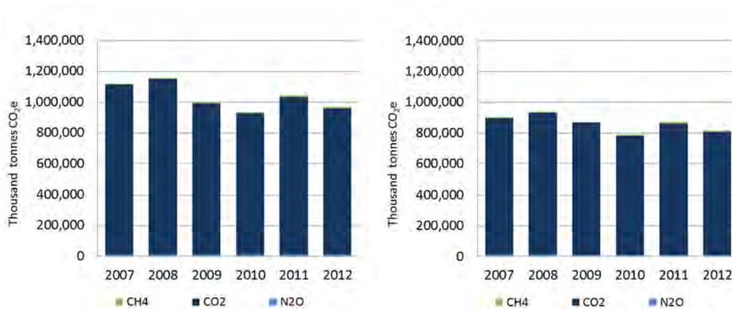
a. Total shipping b. International shipping Figure 41 Time series of bottom-up CO 2 e emissions estimates for a) total shipping, b) international shipping.
