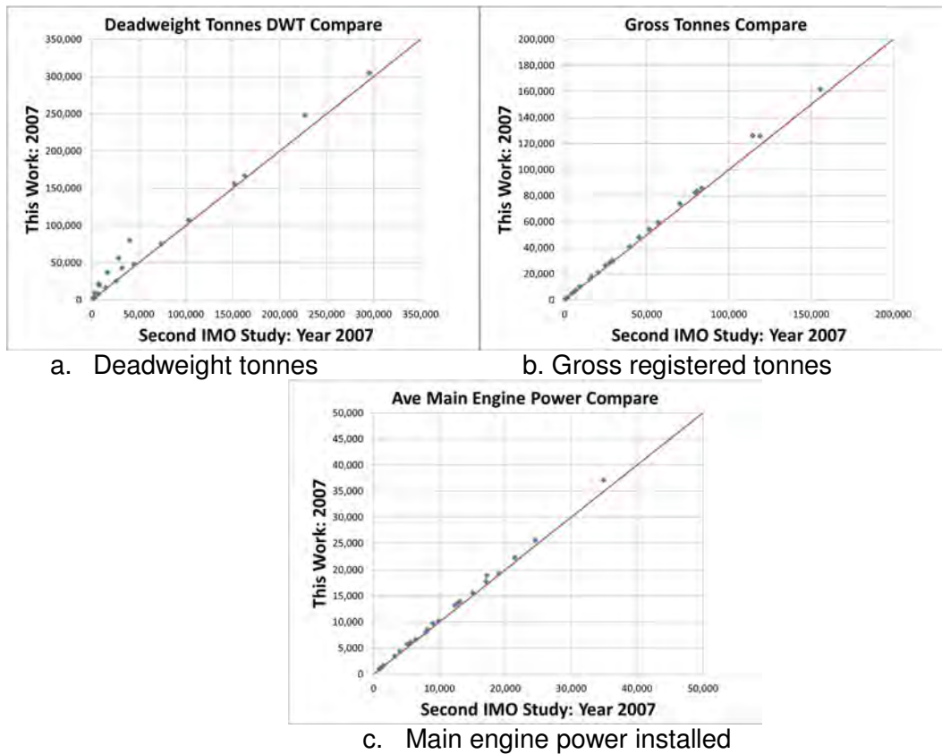
Figure 67 Crossplots of deadweight tonnes, gross tonnes and average installed main engine power for the year 2007, as reported by the IMO GHG Study 2009 (x-axis) and the IMO GHG Study 2014 (y-axis).
