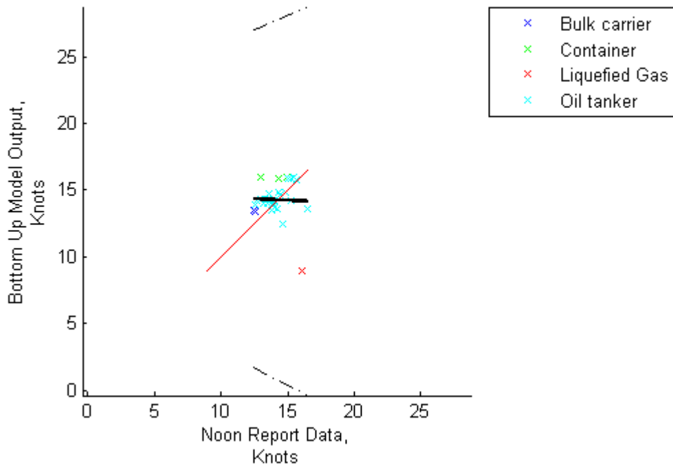
Noon Report Comparison With Bottom Up Output: Average Ship Speed (At Sea)
