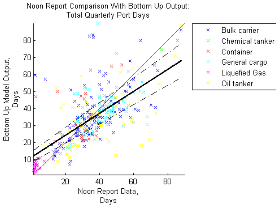
Figure 49 Comparison of at-sea and at-port days are calculated from both the bottom-up model output (y-axis) and the noon report data (x-axis) (2012).
