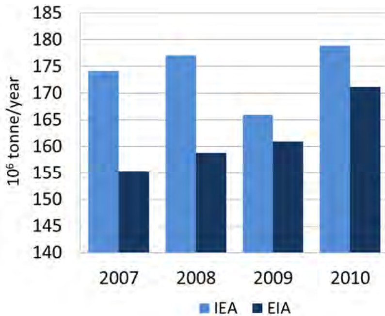
Figure 44 Comparison of IEA and EIA international marine bunker fuel oil statistics.
