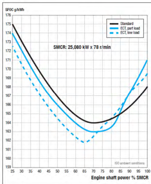
Figure 72 Impact of engine control parameter changes (ECT) to specific fuel oil consumption during low load operation of MAN 6S80ME-C8.2. Standard tuning is shown by the solid black line, part load optimisation by the solid blue line and low load tuning by the broken line (from MAN 2012).
