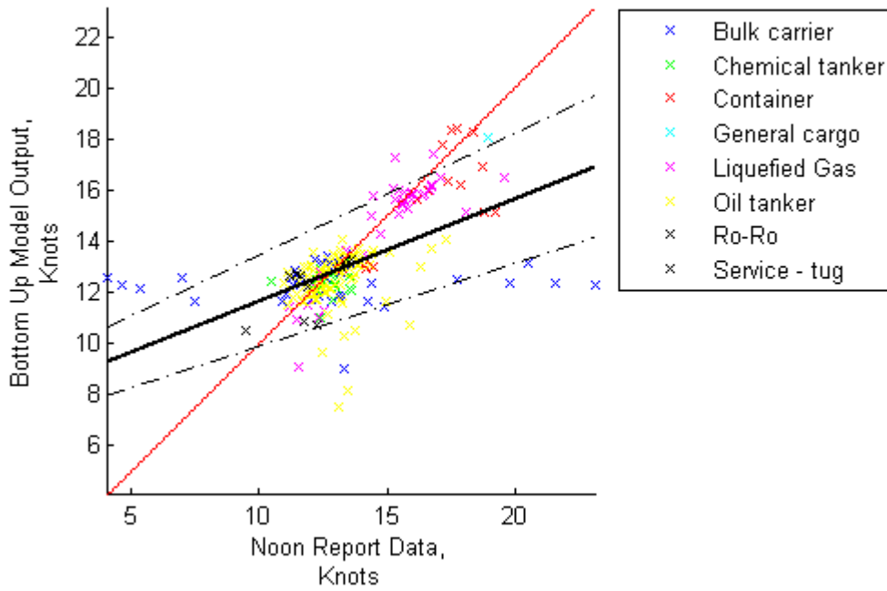
Noon Report Comparison With Bottom Up Output: Average Ship Speed (At Sea)
