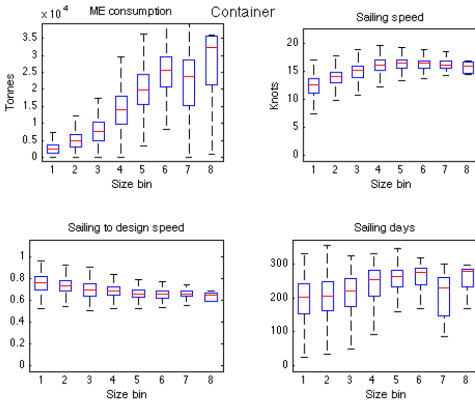
Figure 39 Variability within ship size categories in the container ship fleet (2012). Size category 1 is the smallest containerships (0–999 TEU) and size category 8 is the largest (14,500+ TEU).
