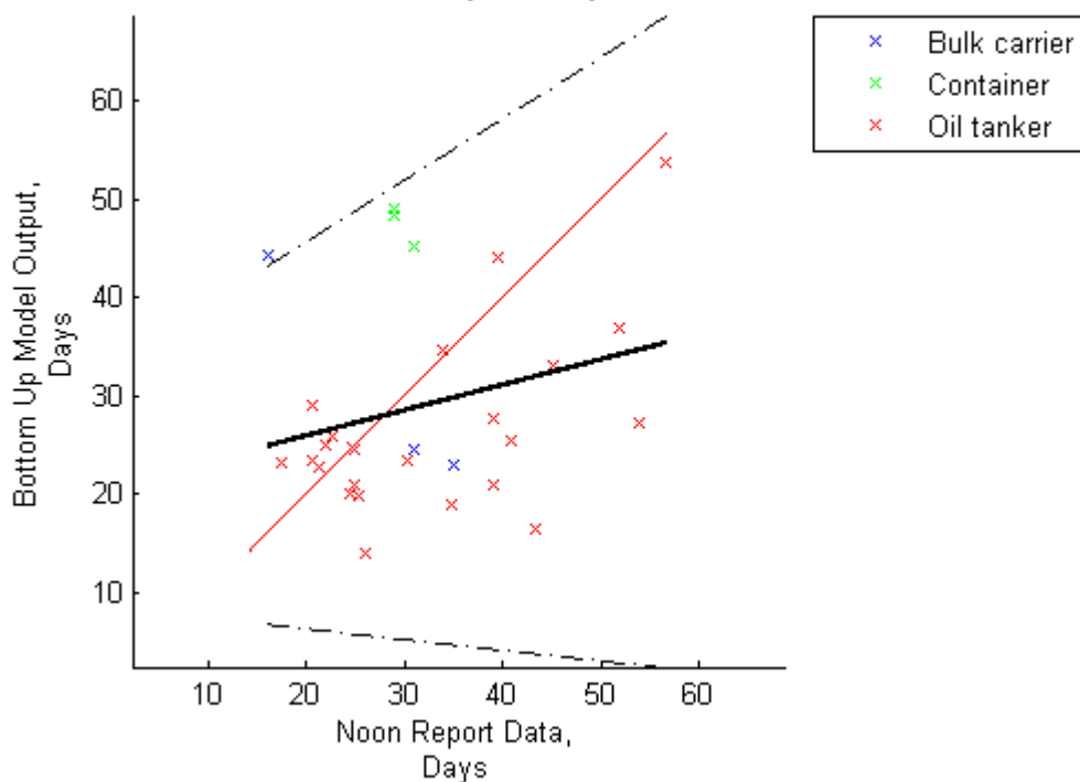
Noon Report Comparison With Bottom Up Output: Total Quarterly Port Days
