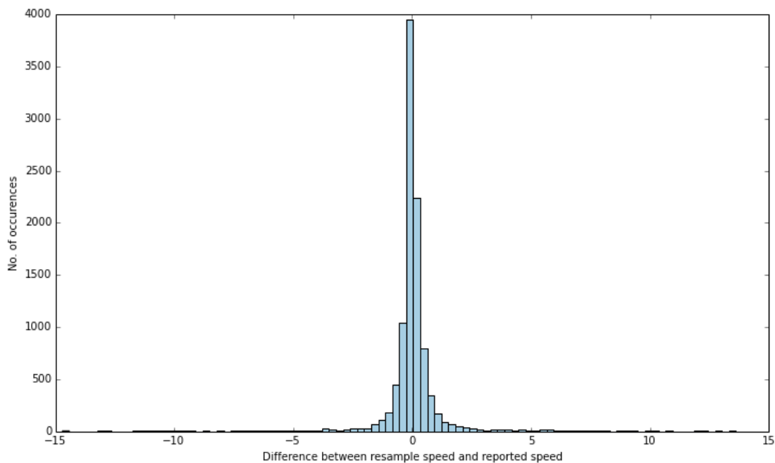
Figure 18: Distribution of difference between reported speeds when the time difference in reporting is between 2hours (sampled as message from 105 mins to 120 mins from the original message) for all VLCC ships captured in AIS. The standard deviation of the sample was 1.85nm/hr.
