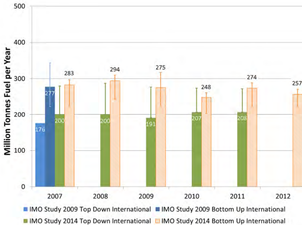
Figure 66 Top-down and bottom-up inventories for international shipping fuels, from the IMO GHG Study 2014 and the IMO GHG Study 2009.
