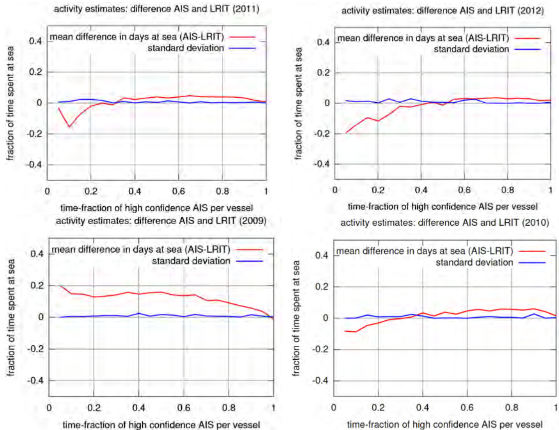
Figure 16: Plots of difference in fraction of time spent at sea for all ships with increasing high confidence AIS count over the year. For each ship in one of these 5%-wide bins, the difference between fraction of time at sea between AIS and LRIT is calculated. The mean of this difference per bin is plotted (red). And the standard deviation of the difference values in each bin is plotted (blue).
