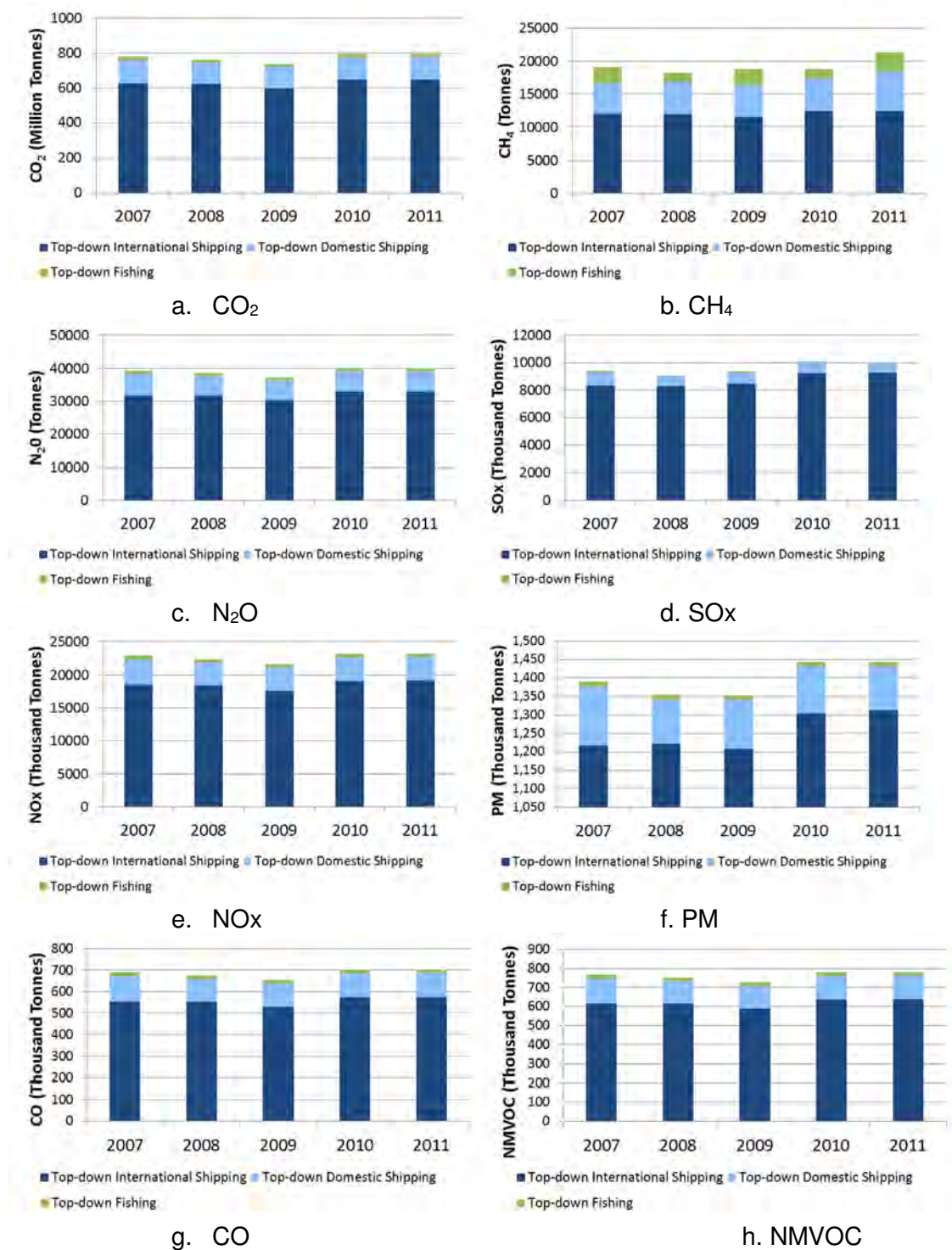
Figure 75 Time series of top-down results for a) CO 2 , b) CH 4 , c) N 2 O, d) SO x , e) NO x , f) PM, g) CO, and h) NMVOC, delineated by international shipping, domestic navigation and fishing.
