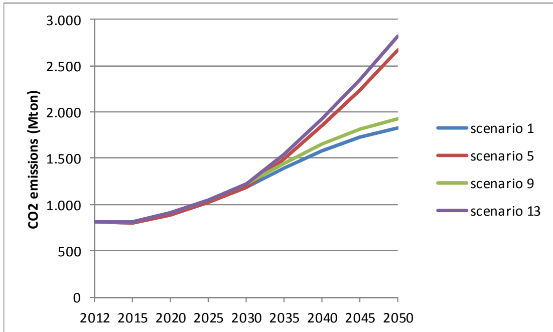
Figure 86 Output for demand scenarios under conditions of high LNG/extra ECA and high efficiency.
