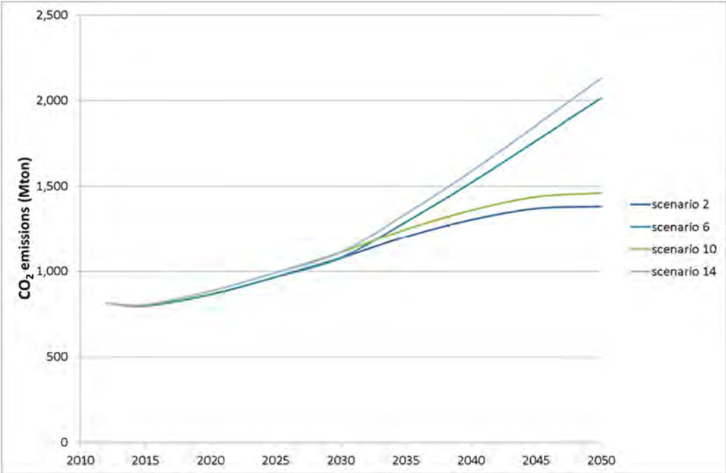
Figure 15: Projections of CO 2 emissions from international maritime transport under the same demand projections. Larger improvements in efficiency have a higher impact on CO 2 emissions than a larger share of LNG in the fuel mix.
