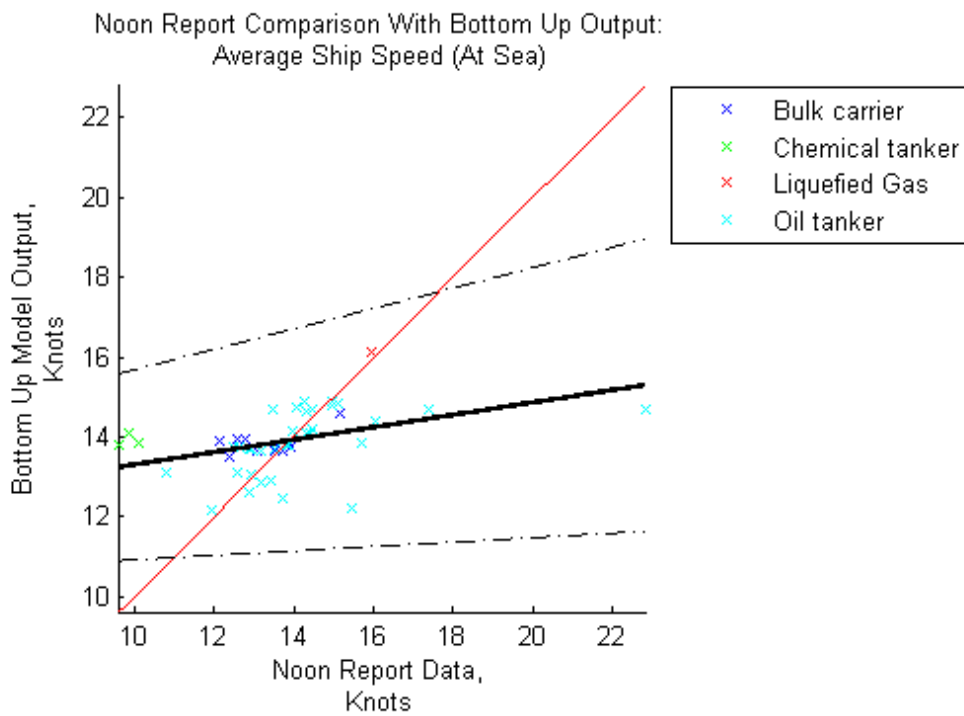
Figure 51 Comparison of at-sea days and average ship speed, calculated from both the bottom-up model output (y-axis) and the noon report data (x-axis) (2009).
