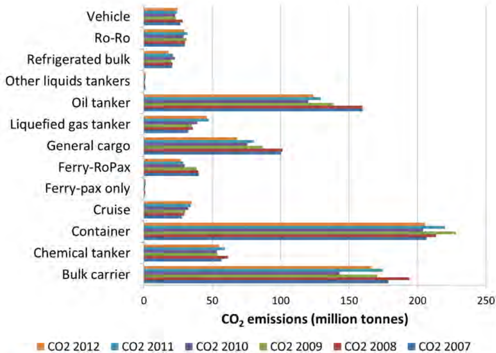
Figure 29 CO 2 emissions by ship type (international shipping only), calculated from the bottom-up method for all years 2007–2012.
