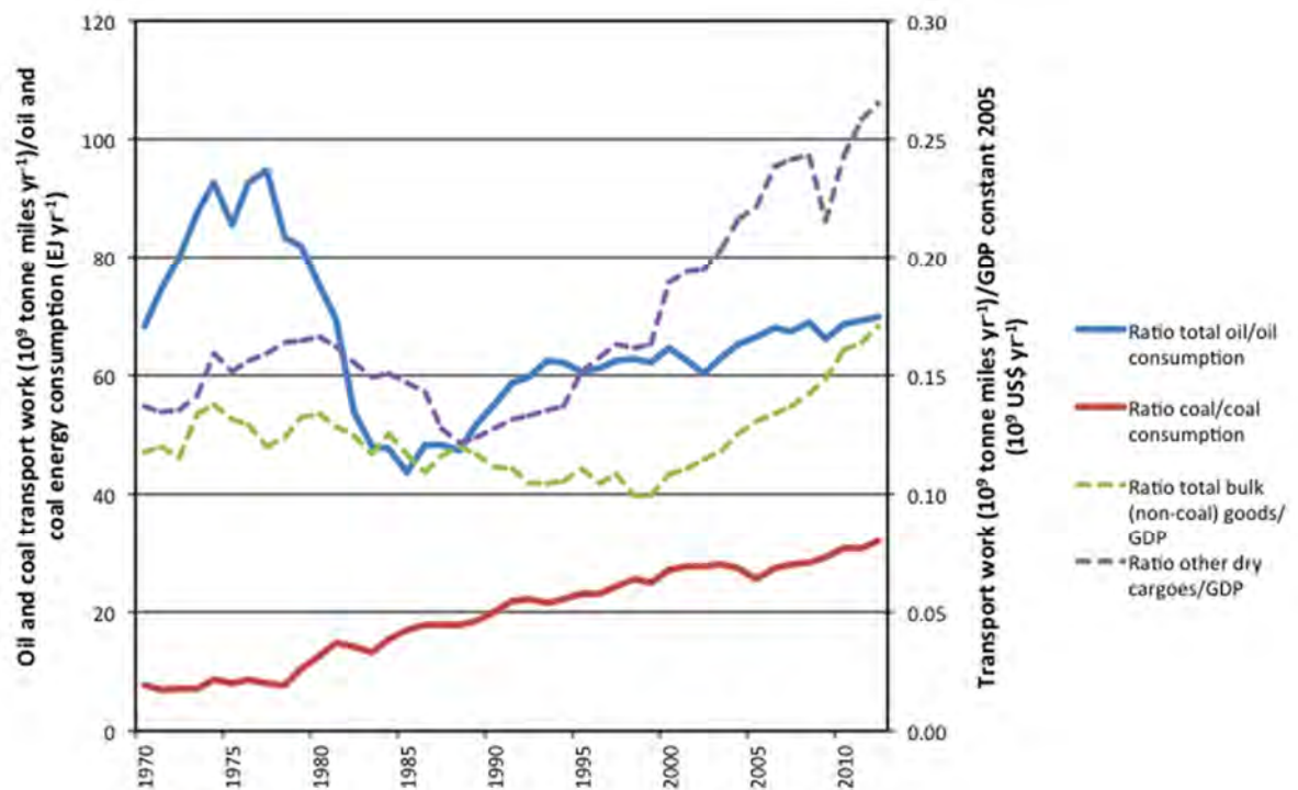
Figure 34: Ratios of TST (different sub-types) in billion tonne-miles to historic global GDP in US$ (constant 2005 prices) and coal/oil consumption (from BP Statistical Review).
