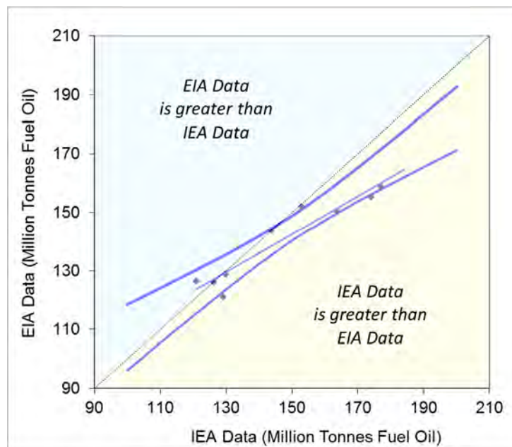
Figure 45 Confidence bands showing statistical difference between IEA and EIA data.
