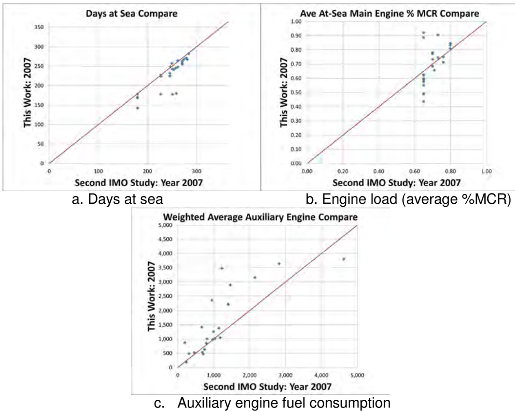
Figure 68 Crossplots for days at sea, average engine load (%MCR) and auxiliary engine fuel use for the year 2007, as reported by the IMO GHG Study 2009 (x-axis) and the IMO GHG Study 2014 (y-axis).
