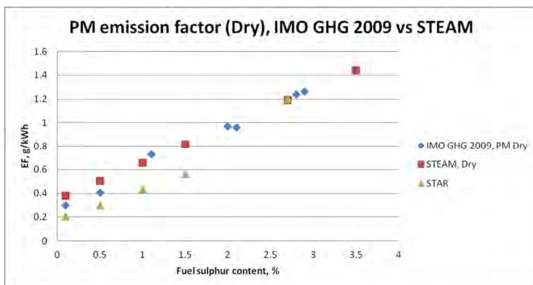
Figure 74 Comparison of PM emissions factors reported in IMO GHG Study 2009 [blue diamond] (Figure 7.7, based on data from Germanischer Lloyd) with values of Jalkanen et al. (2012) [red square] and with Starcrest (2013) [green triangle].
