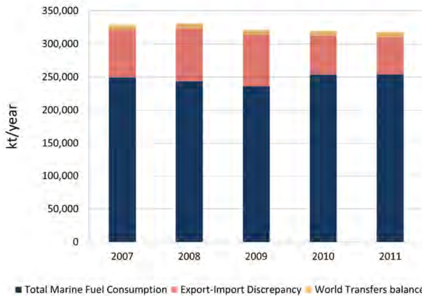
Figure 63 Adjusted marine fuel sales based on quantitative uncertainty results (2007–2011).
