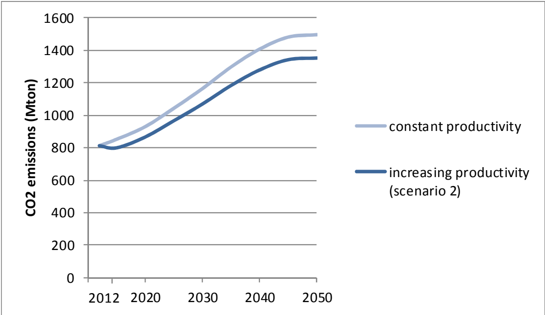
Figure 88 Impact of productivity assumptions on emissions projections.
