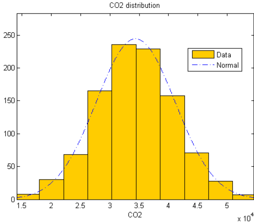
Figure 30: Uncertainty around the annual emissions (x axis is '00000 tonnes of CO 2 ), y axis is frequency, from a Monte Carlo simulation of an 'average' panamax bulk carrier (60-99,999 dwt capacity) in 2007.
