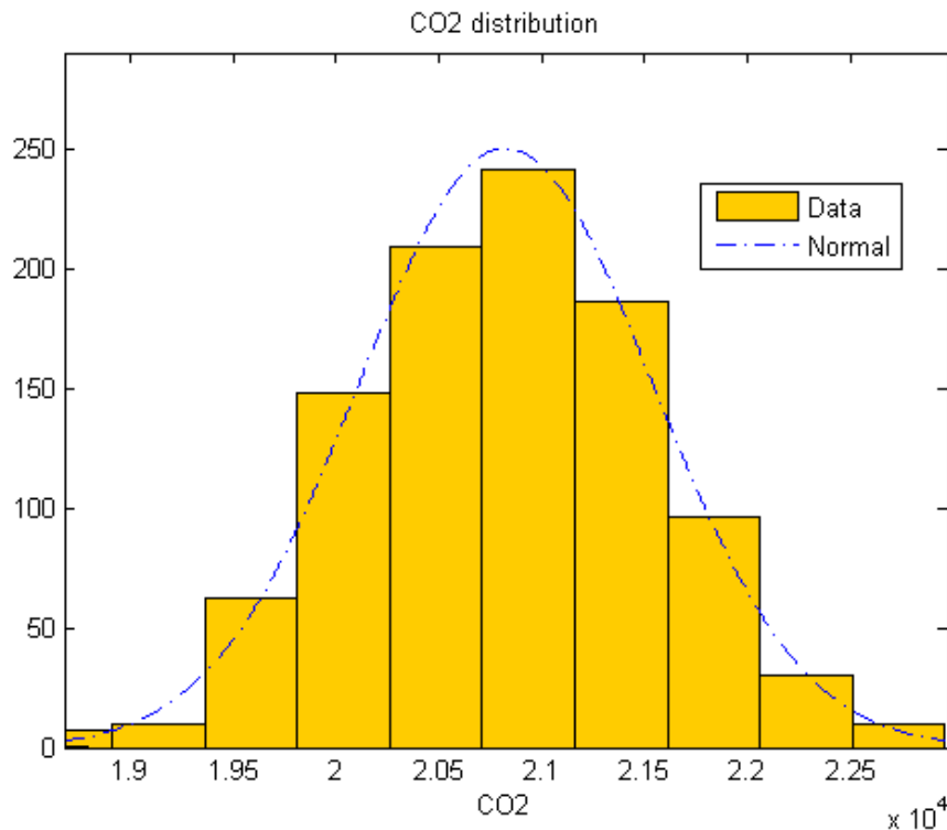
Figure 31: Uncertainty around the annual emissions (x axis is '00000 tonnes of CO 2 ), y axis is frequency, from a Monte Carlo simulation of an 'average' panamax bulk carrier (60-99,999 dwt capacity) in 2012.
