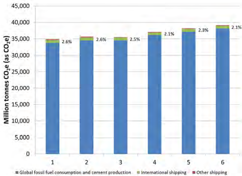
Figure 42 Comparison of shipping with global totals: a) CO 2 emissions compared, where percent shows international shipping emissions CO 2 as a percent of global CO 2 from fossil fuels; b) CO 2 e emissions compared, where percent shows international shipping emissions CO 2 e as a percent of global CO 2 e from fossil fuels.
