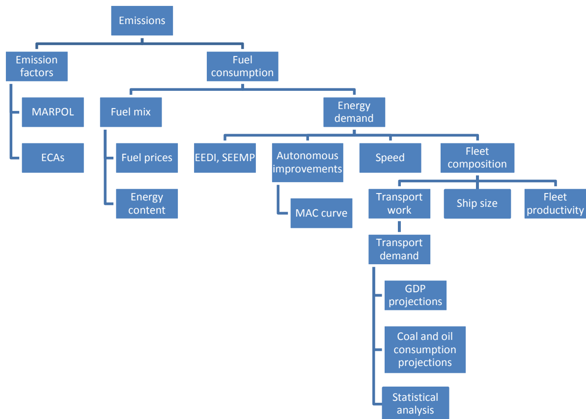
Figure 32: Schematic presentation of emissions projection model
