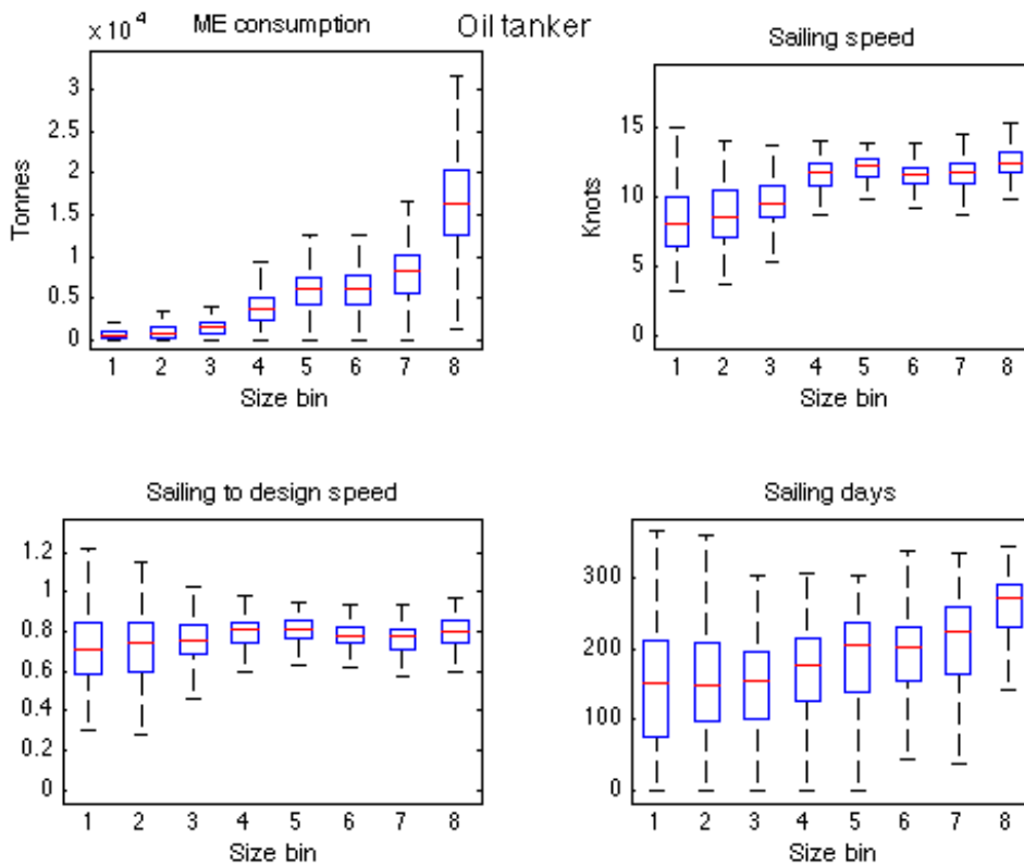
Figure 40 Variability within ship size categories in the tanker fleet (2012). Size category 1 is the smallest oil tankers (0–9999dwt capacity) and size category 8 is the largest (200,000+dwt capacity).
