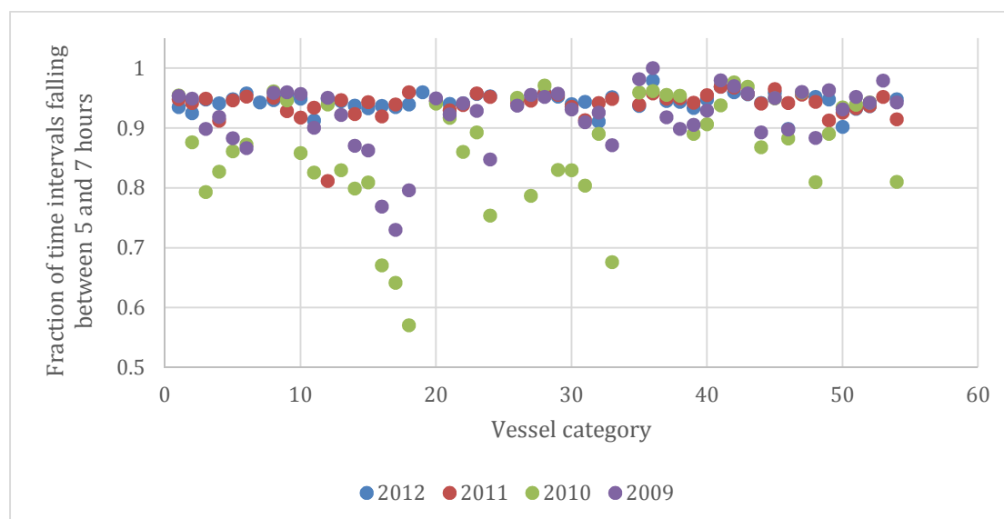
Figure 15: fraction of time intervals between consecutive messages that fall between 5 and 7 hours for each ship type and size category. 1
