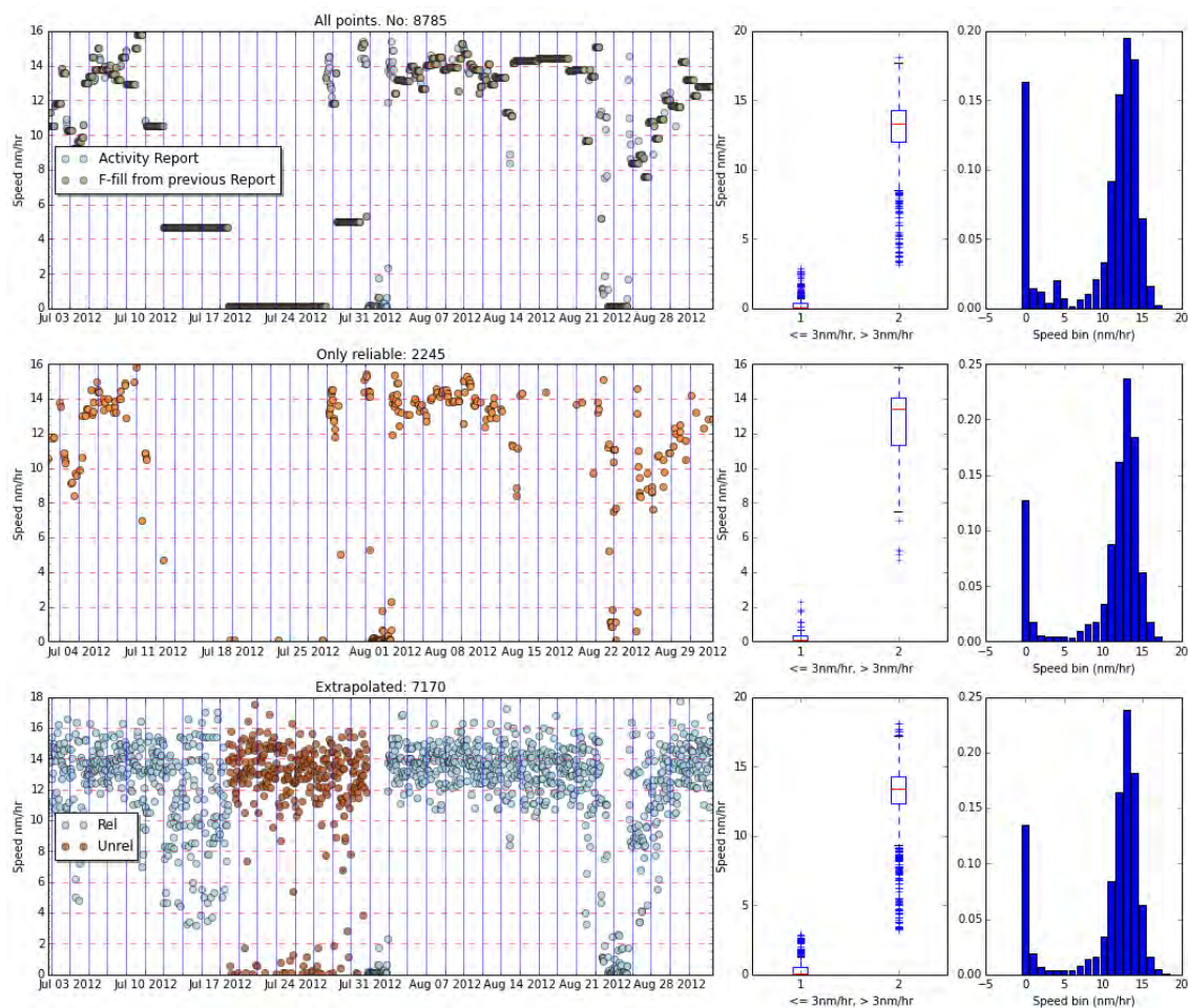
Figure 8: Illustration of the extrapolation process.
