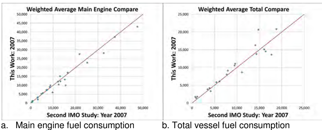
Figure 69 Crossplots for average main engine daily fuel consumption and total vessel daily fuel consumption for 2007, as reported by the IMO GHG Study 2009 (x-axis) and the IMO GHG Study 2014 (y-axis).
