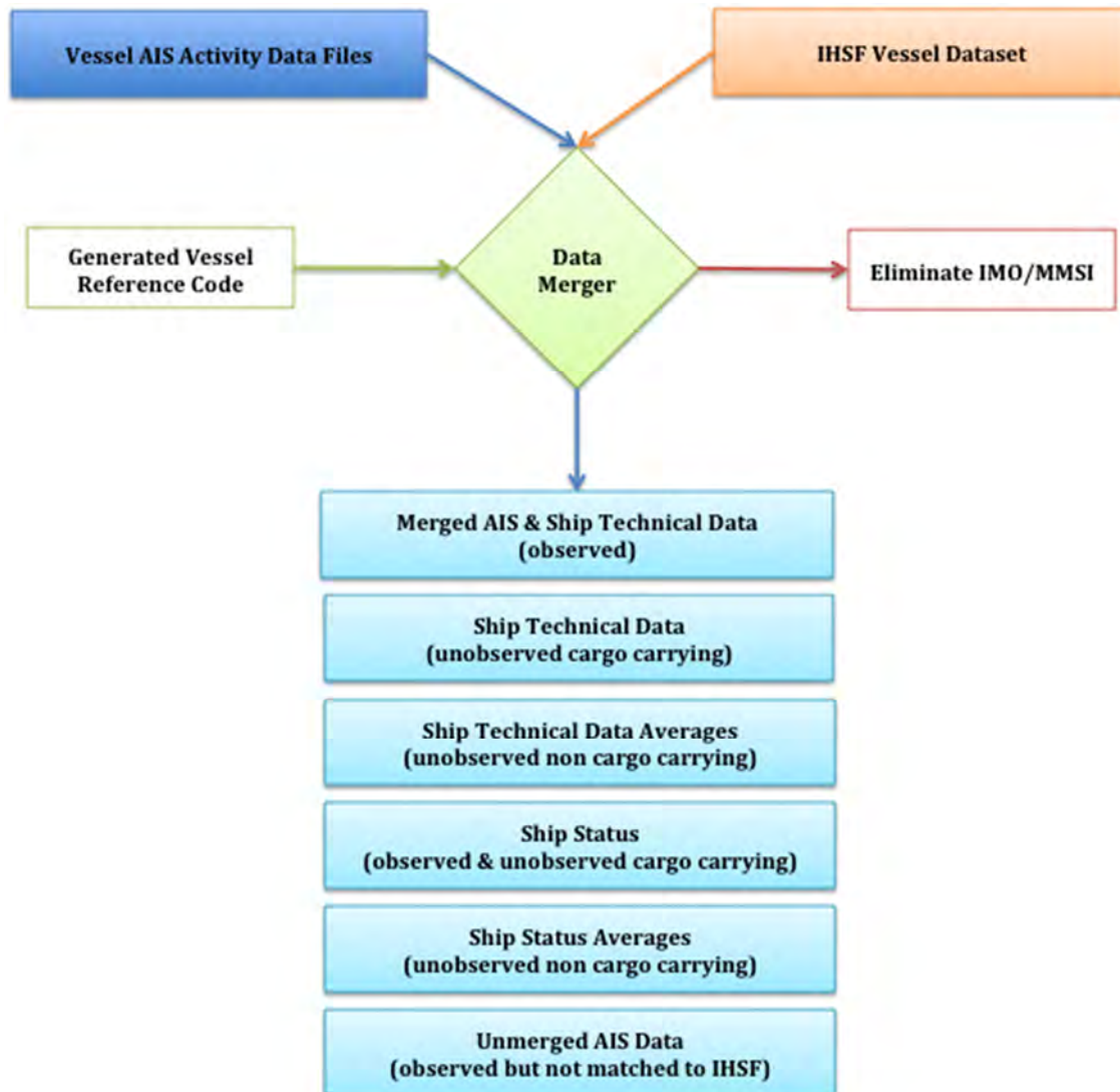
Figure 9: Activity and ship technical and operational data merger process.
