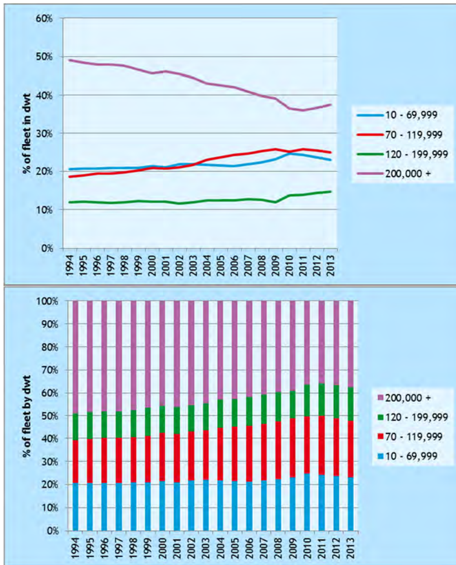
Figure 45: Capacity distribution of tankers over size categories.
