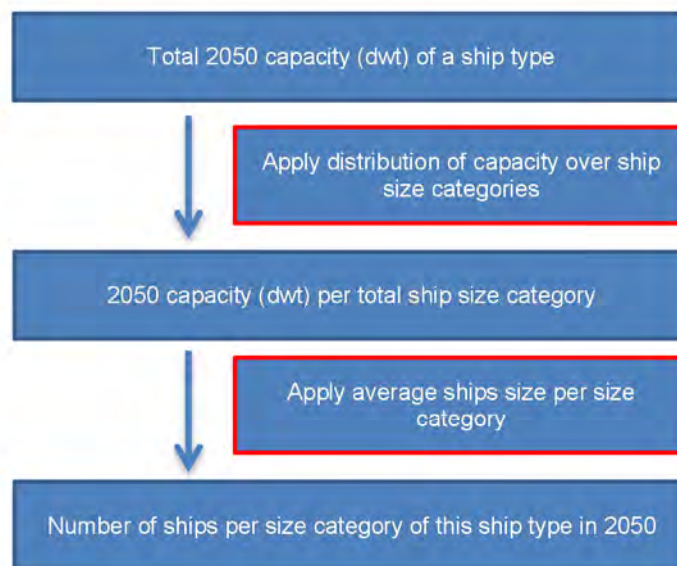
Figure 40: First methodology to determine the number of ships per size category in 2050.
