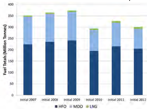
b. Initial bottom-up allocation
