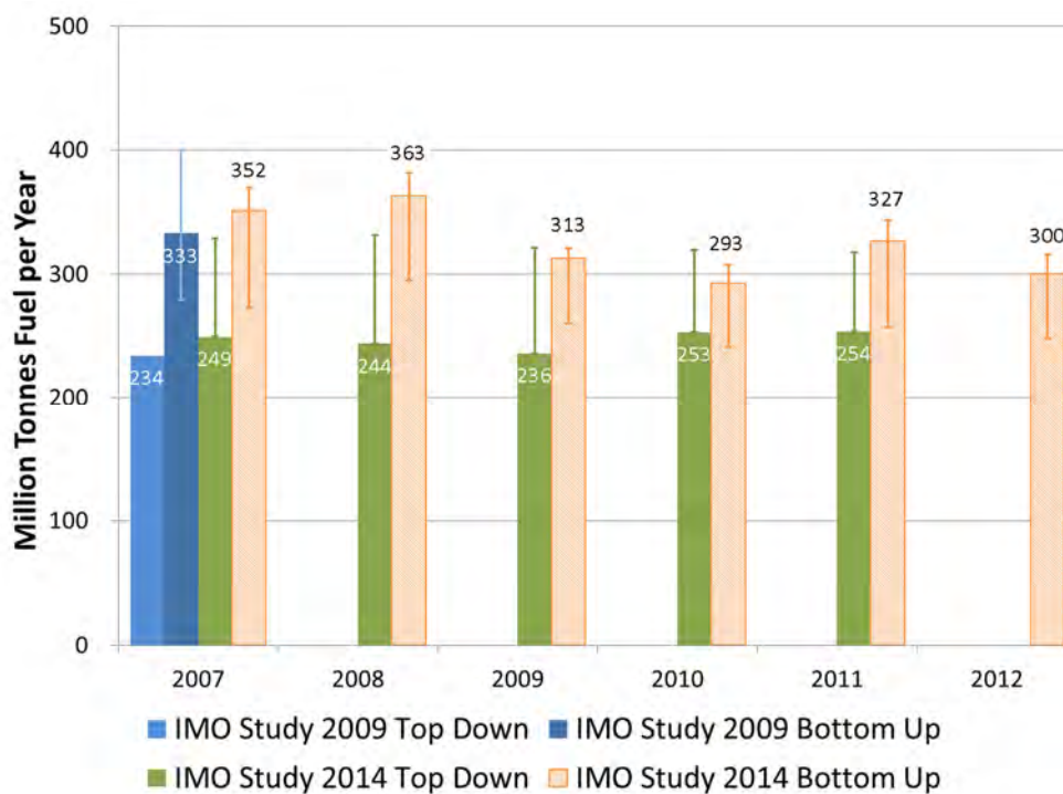
Figure 65 Top-down and bottom-up inventories for all ship fuels, from the IMO GHG Study 2014 and the IMO GHG Study 2009.
