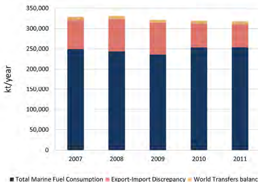
Figure 25: 2007-2011 adjusted marine fuel sales based on quantitative uncertainty results.
