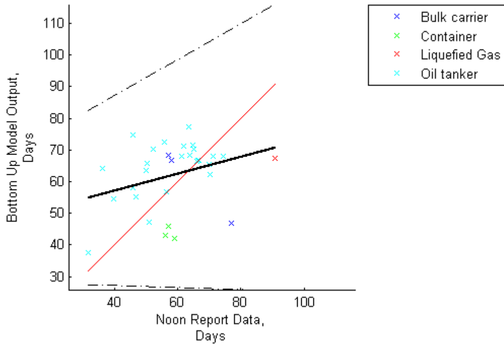
Noon Report Comparison With Bottom Up Output: Total Quarterly At Sea Days
